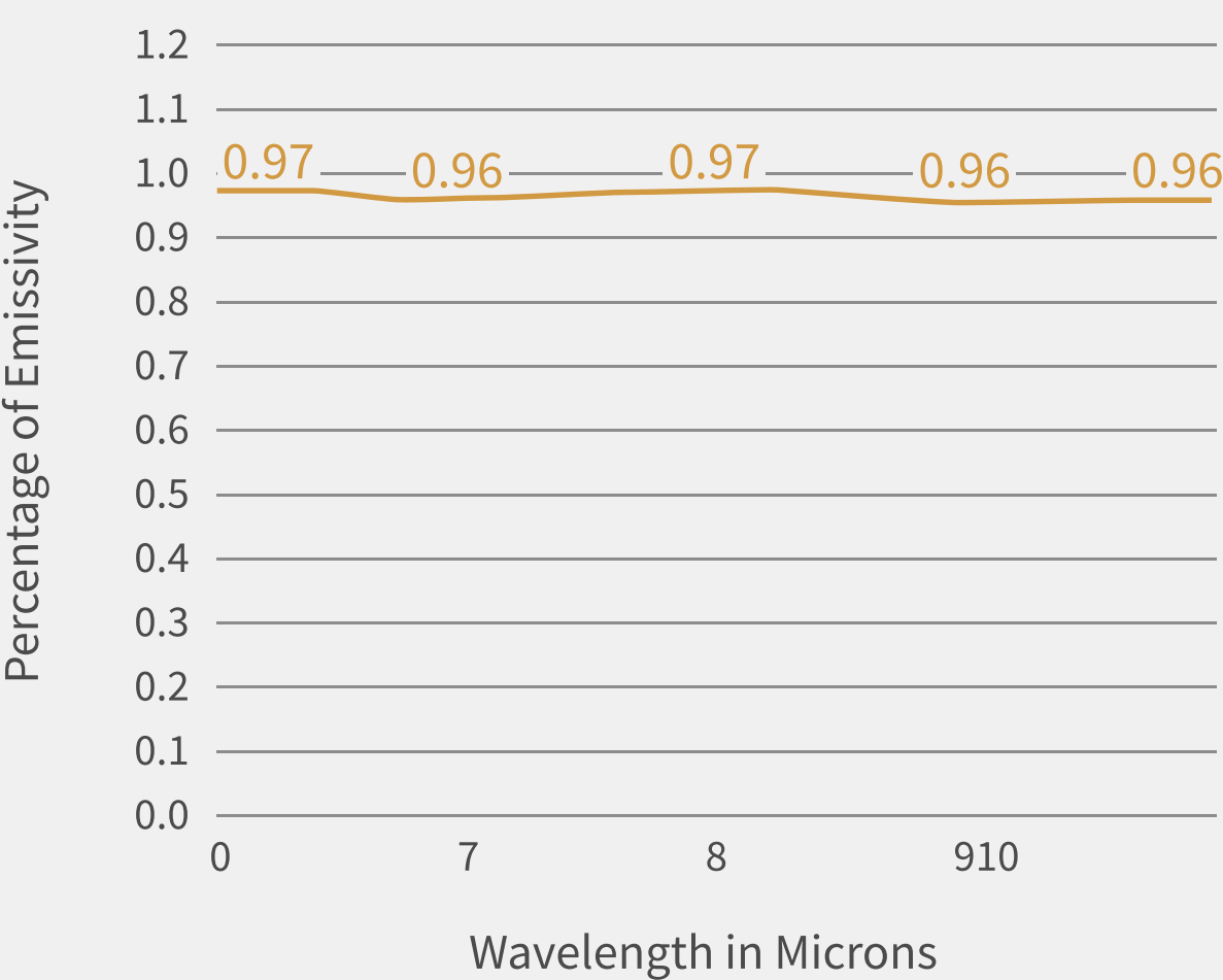
Emissivity Test Results:
